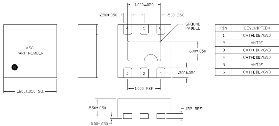
Figure 7 Package Outline
