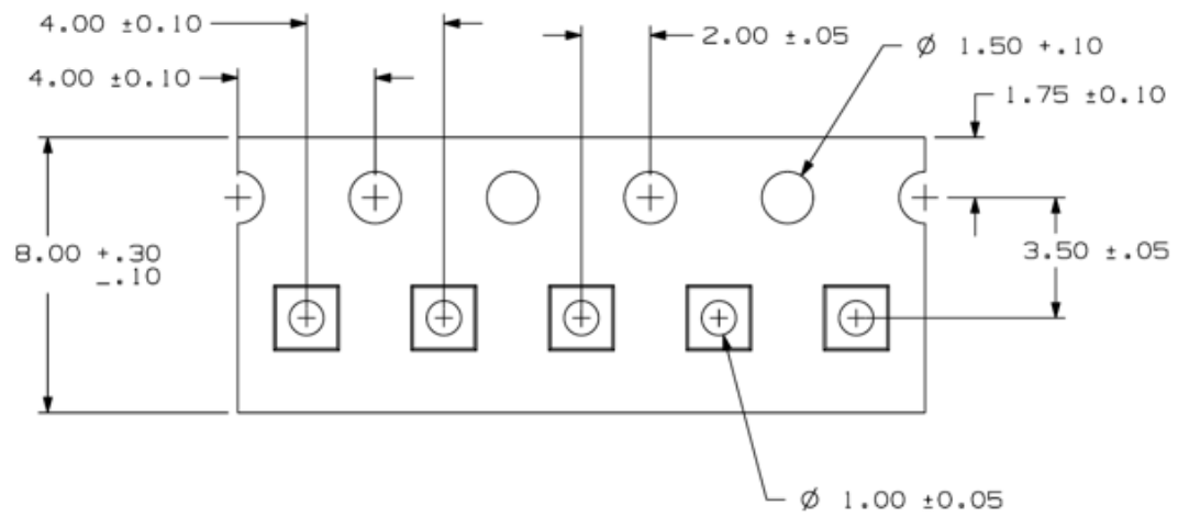
Figure 9 Tape-and-Reel Format
