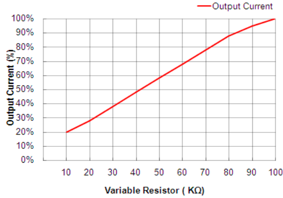
Output Current vs. Variable Resistor
