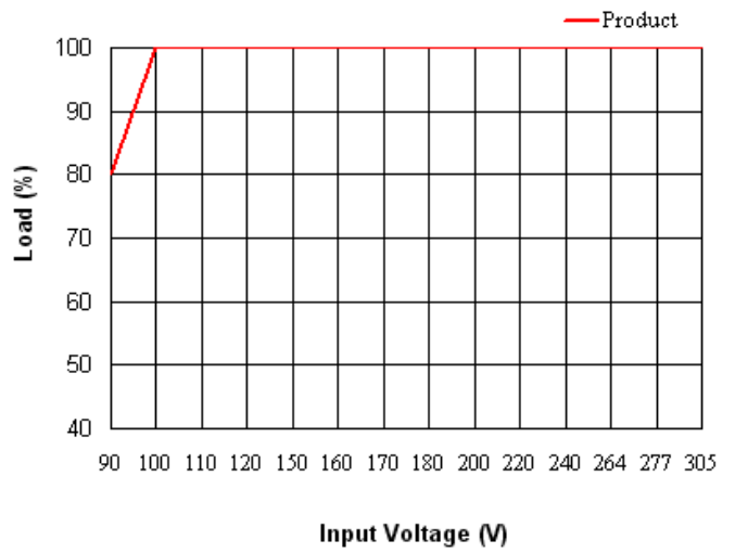
Static Curve
