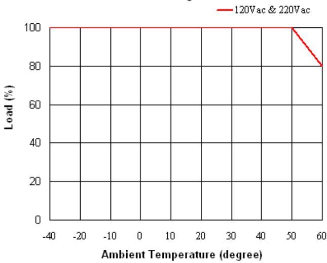
Derating Curve
