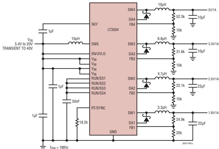
Quad Buck Regulator in 4 × 5 QFN
