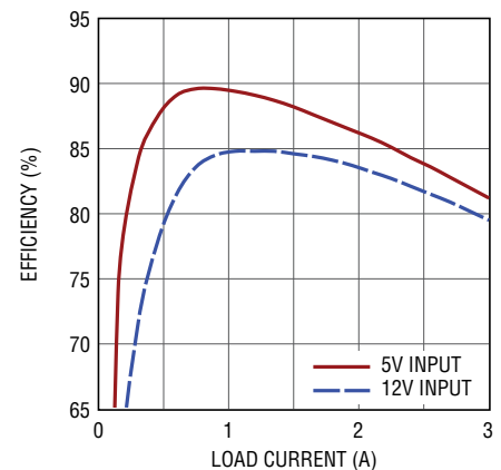
Output Efficiency vs Load Current
