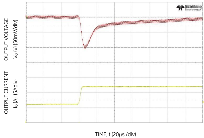
Figure 34. Transient Response to Dynamic Load Change from 50% to 100% at 12Vin, C_{out}=6 \times 47 \mu F , C_{Tune}=1200pF , R_{Tune}=300
