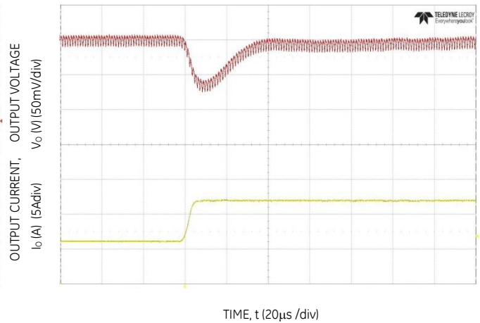
Figure 28 Transient Response to Dynamic Load Change from 50% to 100% at 12V in , C out =3x47μF+1x330μF, C Tune =1800pF, R Tune =300
