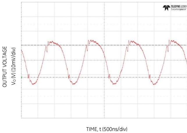
Figure 33. Typical output ripple and noise ( C_o=2 \times 47 \mu F ceramic, V_{IN} = 12V , I_o = I_{o,max} , 20MHz BW).
