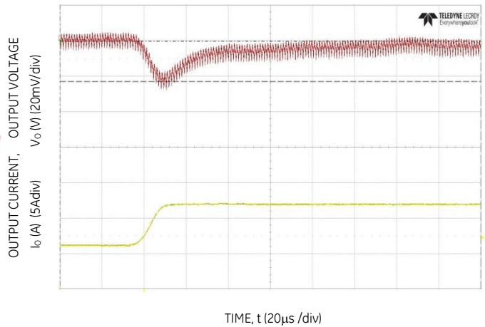
Figure 16. Transient Response to Dynamic Load Change from 50% to 100% at 12V in , C out =4x47µF+2x330µF, C Tune =8.2nF, R Tune =300
