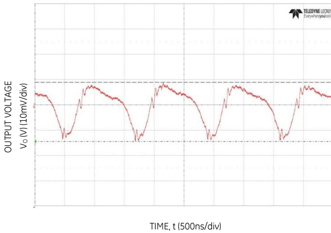
Figure 21. Typical output ripple (Co=2x47µF ceramic, VIN = 12V, Io = Io,max, 20MHz BW).
