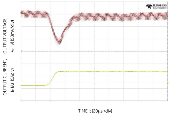
Figure 22. Transient Response to Dynamic Load Change from 50% to 100% at 12Vin, Cout=4x47uF+1x330uF, CTune=2700p, RTune=300
