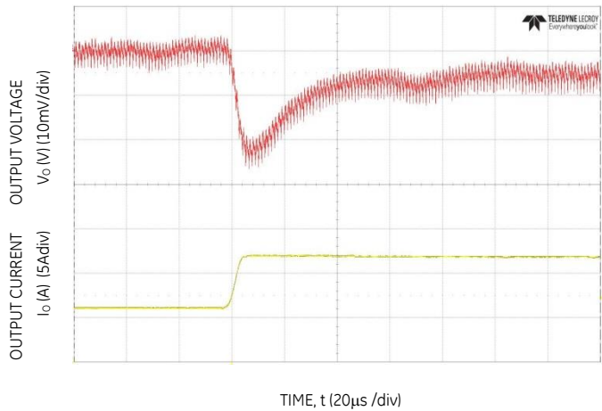
Figure 10. Transient Response to Dynamic Load Change from 50% to 100% at 12Vin, Cout=4x47µF+3x330µF, CTune=10nF, RTune=300
