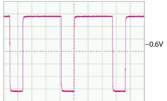
10 ns/DIV, 200mV/DIV
