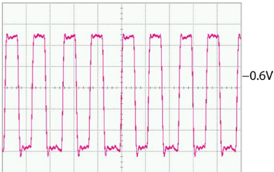
500 ps/DIV, 200mV/DIV
