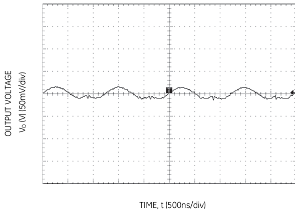
Figure 15. Typical output ripple and noise ( C_o=2 \times 47 \mu F ceramic, V_{IN} = 12V , I_o = I_{o,max} ).
