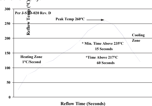
Figure 51. Recommended linear reflow profile using Sn/Ag/Cu solder.
