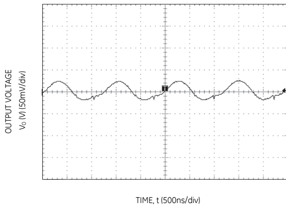
Figure 27. Typical output ripple and noise ( C_o=2 \times 47 \mu F ceramic, V_{IN} = 12V , I_o = I_{o,max} ).
