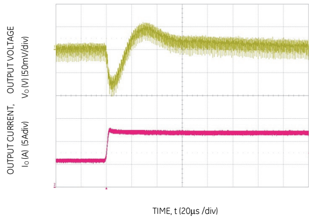
Figure 28. Transient Response to Dynamic Load Change from 50% to 100% at 12Vin, C_{out} = 2 \times 47 \mu F + 1 \times 330 \mu F , C_{Tune}=2700pF & R_{Tune}=300\Omega
