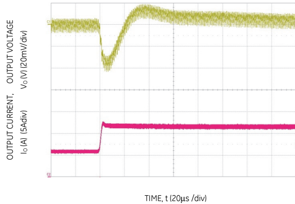
Figure 16. Transient Response to Dynamic Load Change from 50% to 100% at 12Vin, C_{out} = 2 \times 47 \mu F + 2 \times 330 \mu F , C_{Tune} = 5600 pF & R_{Tune} = 220 \Omega
