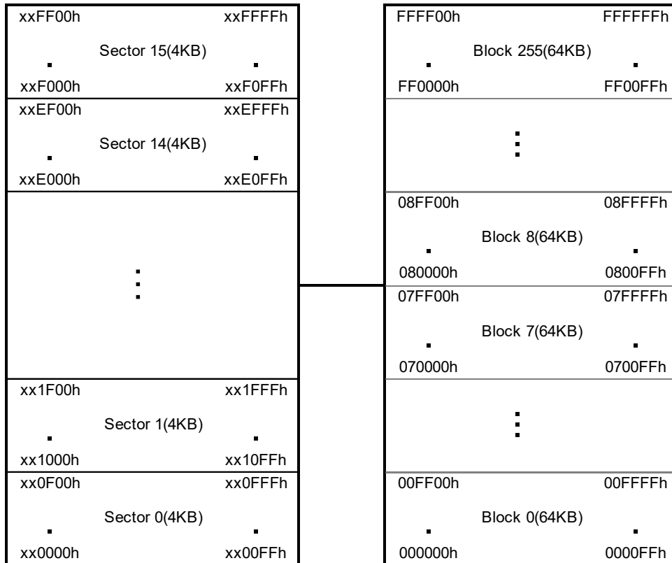
Figure 4, Memory Organization
