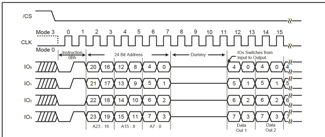
Figure 14b. Fast Read instruction (QPI Mode, 80MHz)
