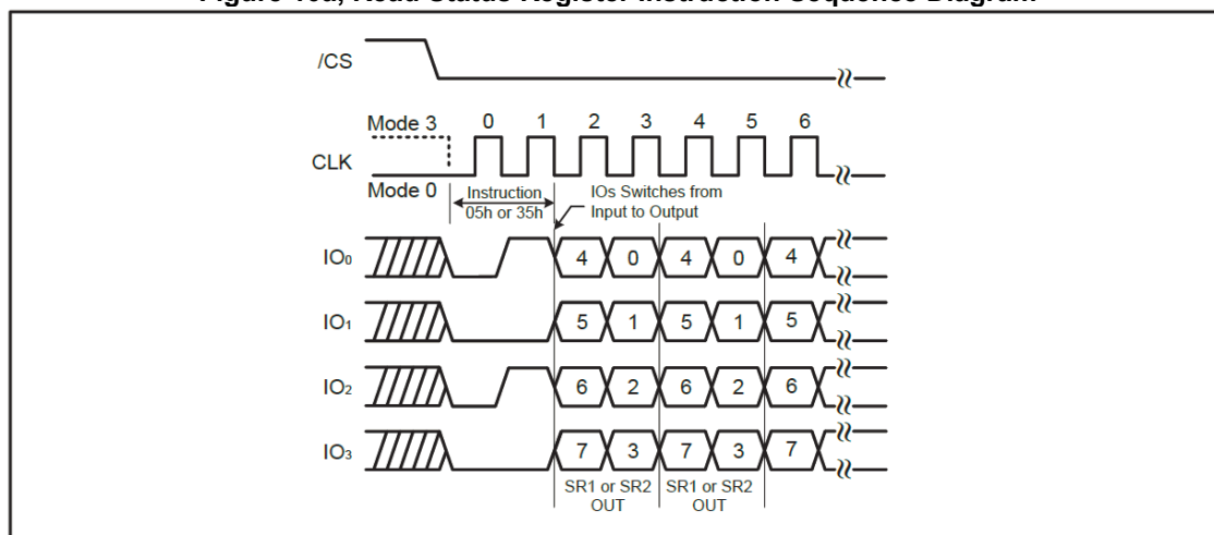
Figure 10b. Read Status Register Instruction (QPI Mode)
