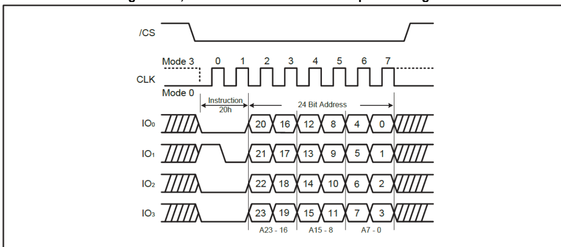
Figure 26b, Sector Erase Instruction Sequence Diagram(QPI Mode)
