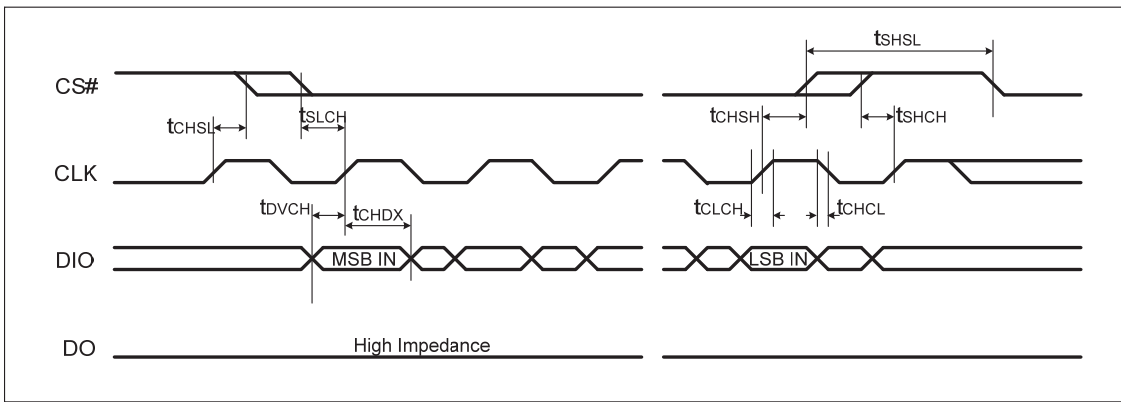
Figure 48, Input Timing
