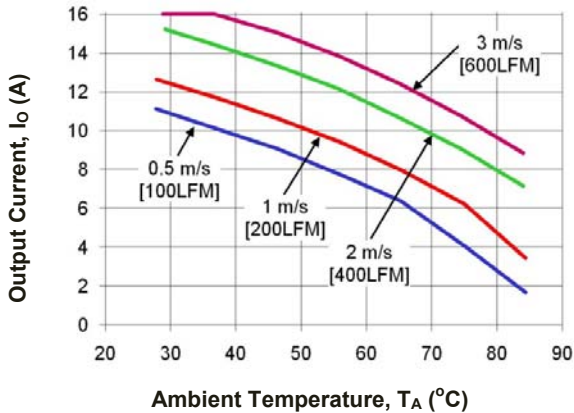
Figure 19. Derating Output Current vs. local Ambient temperature and Airflow, No Heatsink, Vin=48V, airflow from Vi(-) to Vi(+).
