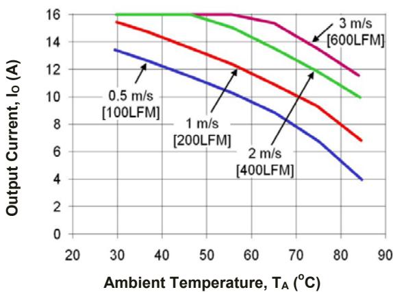
Figure 20. Derating Output Current vs. local Ambient temperature and Airflow, 0.5" Heatsink, Vin=48V, airflow from Vi(-) to Vi(+).
