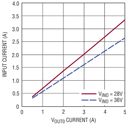
Input Current vs Output Current, V_{\text{OUTO}} = 18\text{V}
