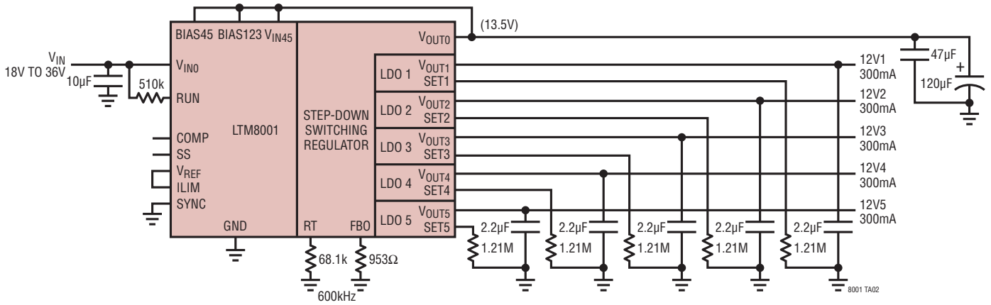
Five Output DC/DC \mu Module Regulator
