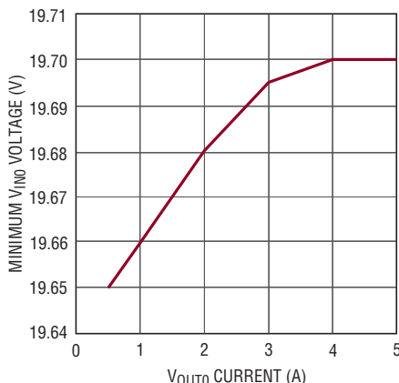
Minimum V_{\text{INO}} vs Output Current, V_{\text{OUTO}} = 18\text{V}
