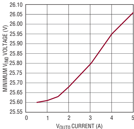
Minimum V_{\text{INO}} vs Output Current, V_{\text{OUTO}} = 24\text{V}
