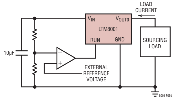
Figure 5d. This Comparator Circuit Turns Off the LTM8001 if the Input Rises Above a Predetermined Threshold. When the LTM8001 Turns Off, the Energy Stored in the Internal Inductor Will Raise V_{IN} a Small Amount Above the Threshold.
