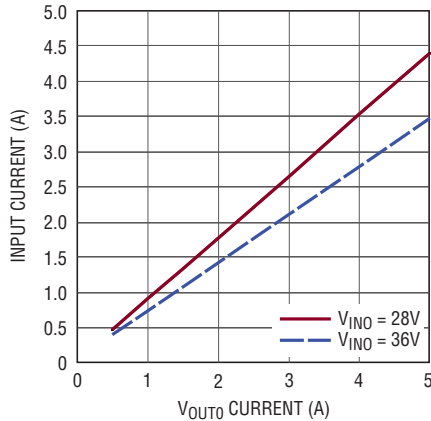
Input Current vs Output Current, V_{\text{OUTO}} = 24\text{V}
