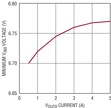
Minimum V_{\text{INO}} vs Output Current, V_{\text{OUTO}} = 5\text{V}
