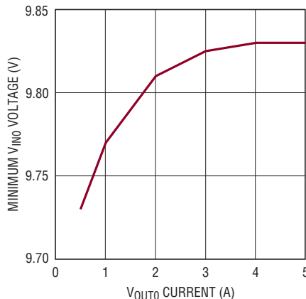
Minimum V_{\text{INO}} vs Output Current, V_{\text{OUTO}} = 8\text{V}
