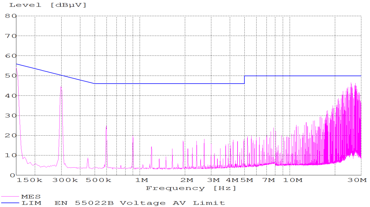
Figure 25. EMC Considerations
