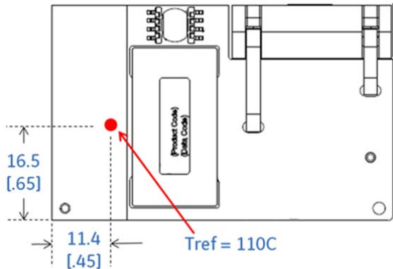
Figure 15. Location of the thermal reference temperature TH 1 for open frame module.
